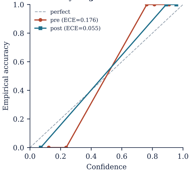
Reliability diagram
