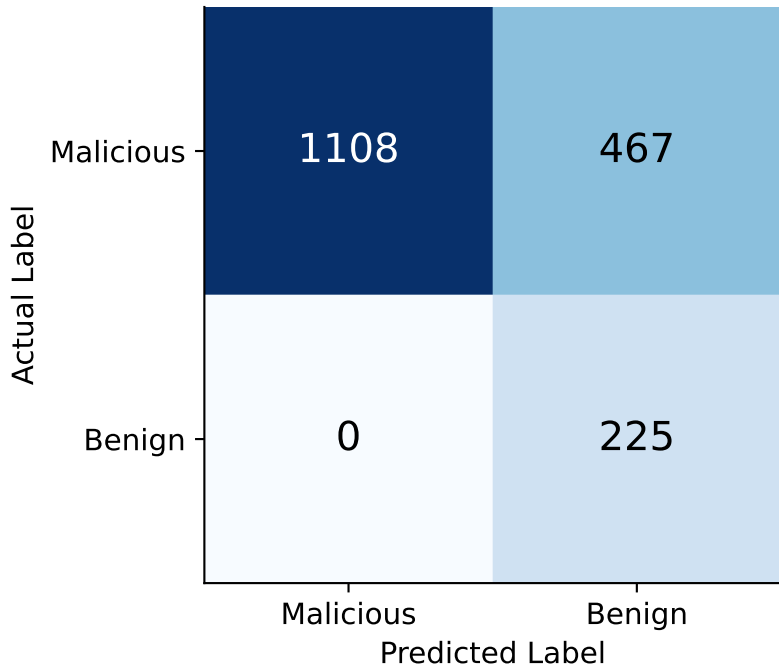
Confusion Matrix (full stack)
