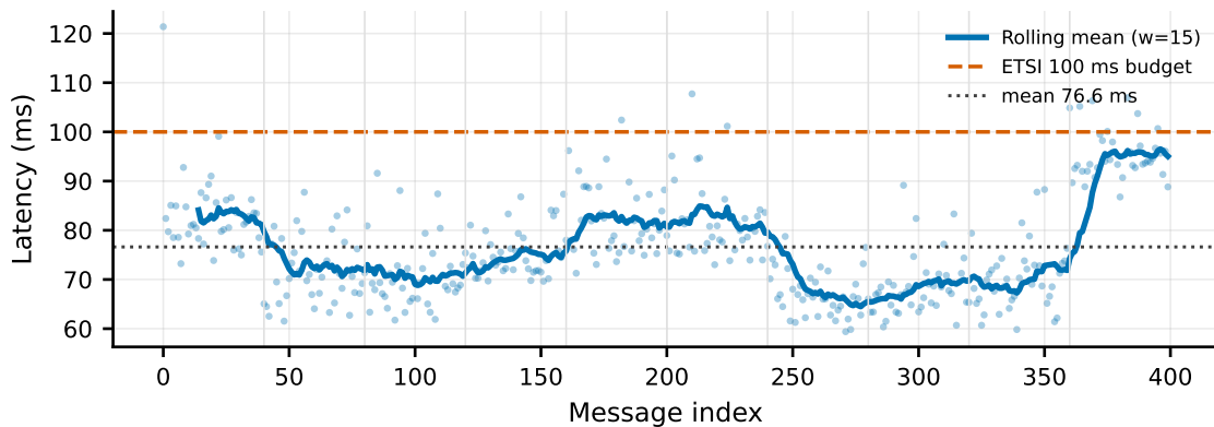
(A) Latency Timeline, Live CARLA, Final Checkpoint ( n = 400 , p_{95} = 95.7 ms)
