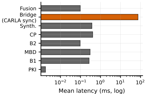
(B) Per-Stage Breakdown (bridge = CARLA sync, not B3)
