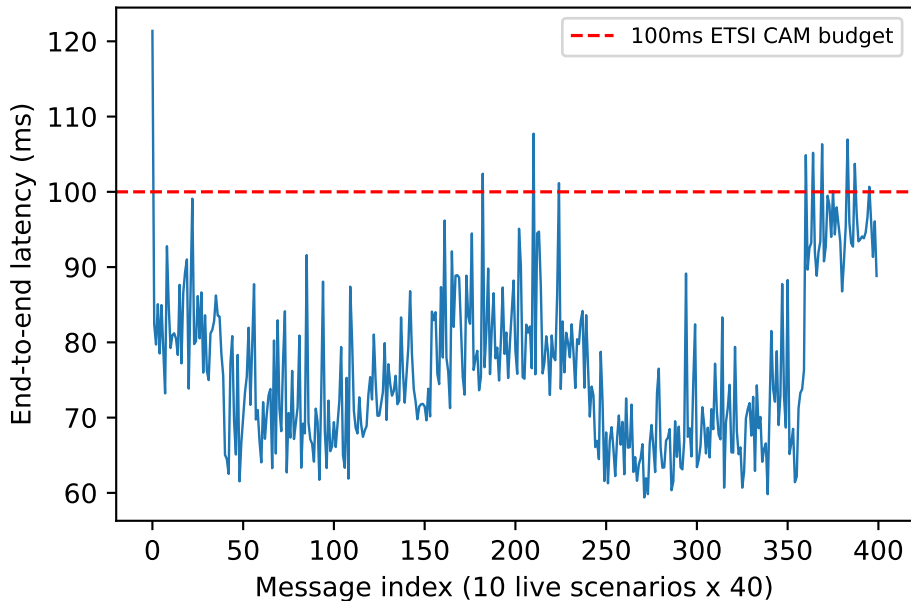
Per-message latency, live CARLA (n=400)
