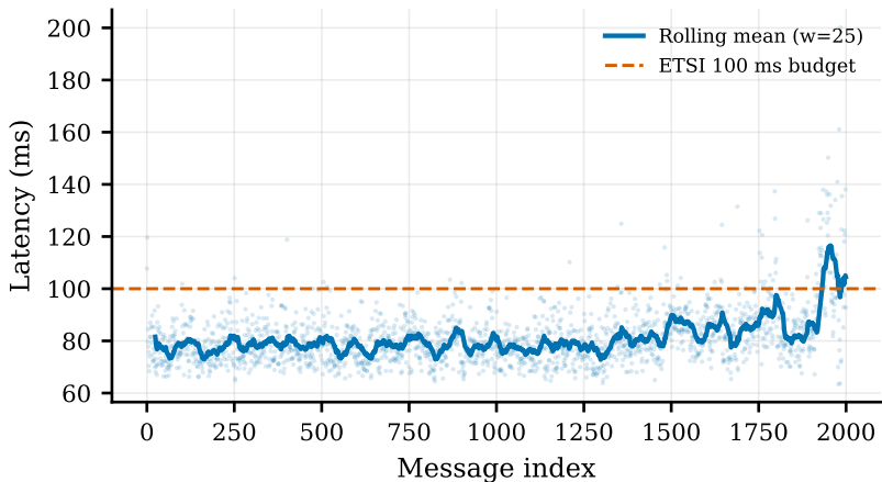
Latency Timeline, SUMO Replay, Prior Checkpoint ( n = 2,000 )
