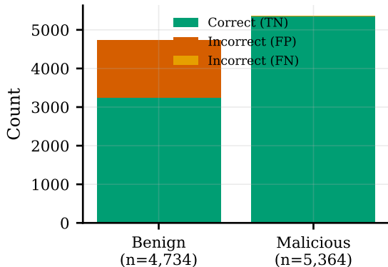
(B) Correct vs. Incorrect by Ground Truth
