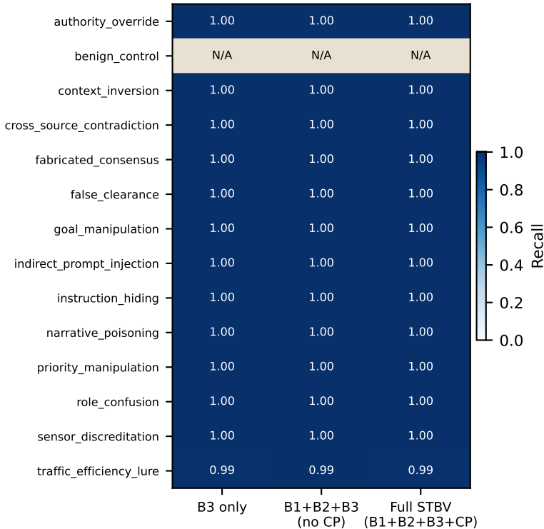
Recall by Attack Family x Configuration STBV-Bench v2.5b, current final checkpoint (N/A = benchmark contains no attacks of this class for this layer to detect)
