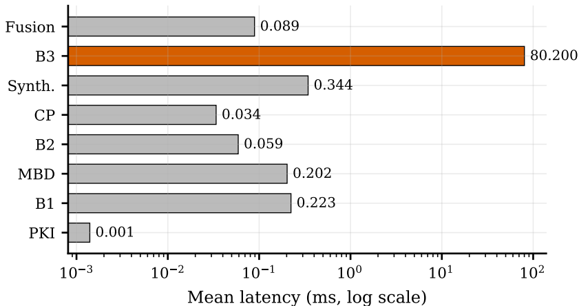
Per-Stage Latency, SUMO Replay Current Final Checkpoint ( n = 2,000 )
