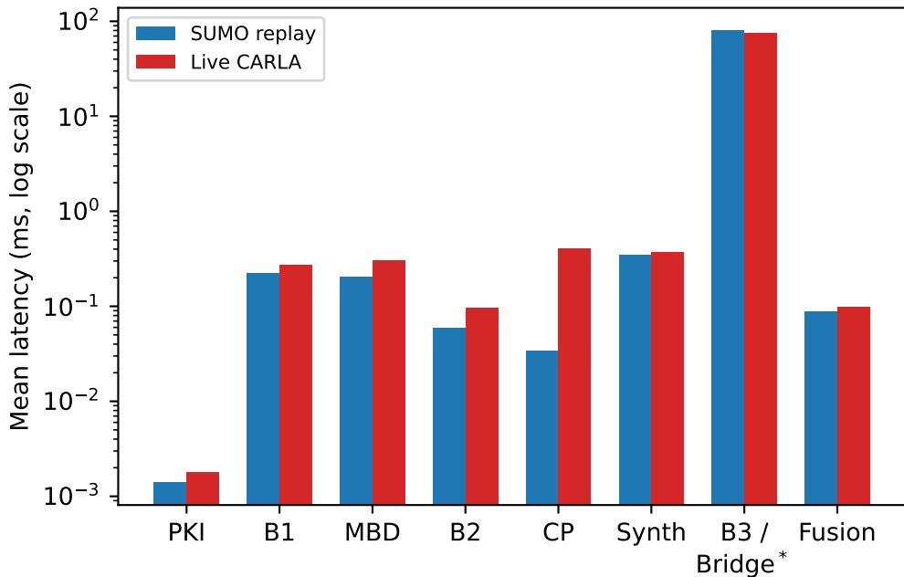
Per-stage latency: replay vs. live CARLA
