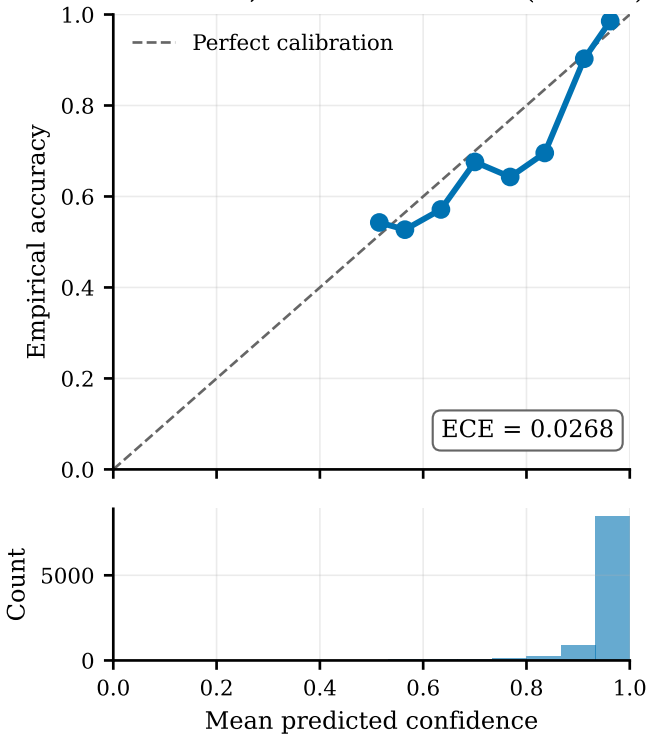
Calibration, STBV-Bench v2.5b (T=3.18)
