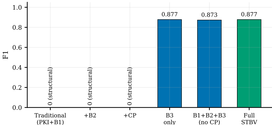
Progressive Layer Contribution, STBV-Bench v2.5b (current final checkpoint; grey bars are a genuine structural zero, not missing data -- see Section~VI-C)
