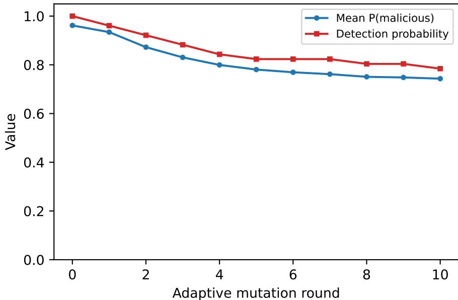
Adaptive-attack confidence/detection, n=51 seeds
