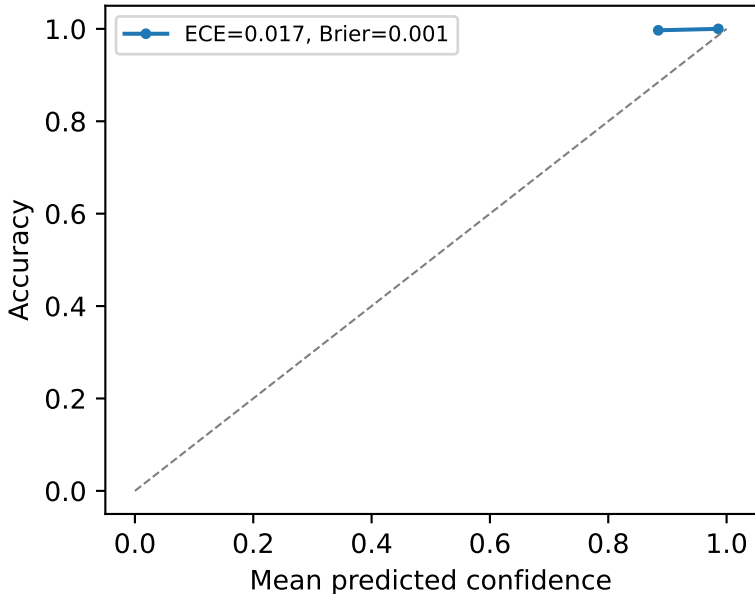
Reliability diagram, B3, STBV-Bench v1
