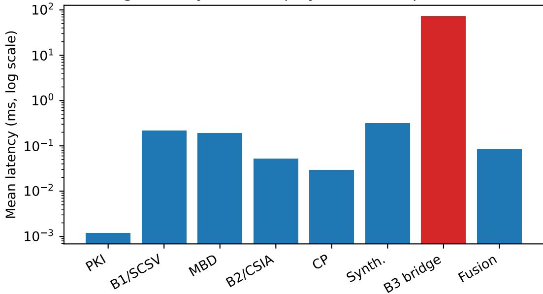
Per-stage latency, SUMO replay, final checkpoint (n=2,000)
