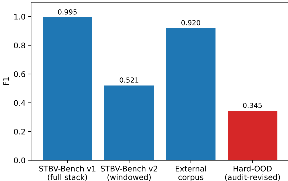
B3 (full stack where applicable) F1 across evaluation regimes
