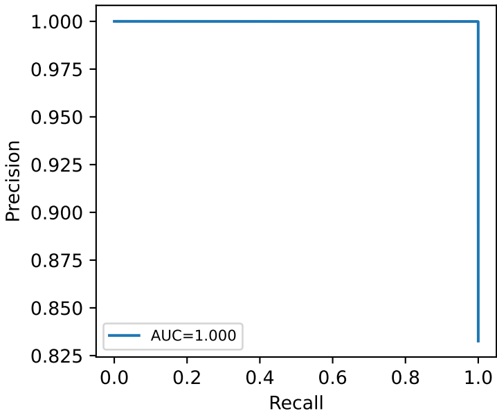
PR curve, full-stack fused score, STBV-Bench
