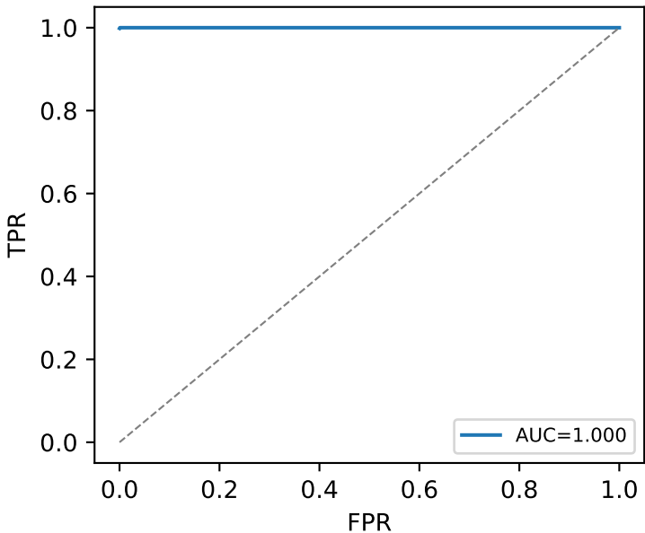
ROC, full-stack fused score, STBV-Bench v1
