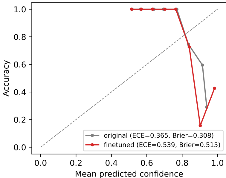
Reliability — B3 alone (config 4), STBV-Bench v
