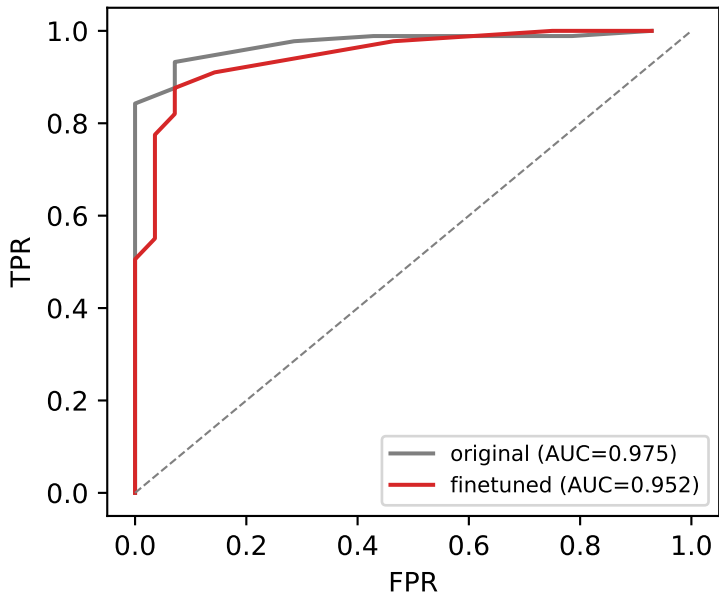
ROC — External Semantic Corpus (n=117)
