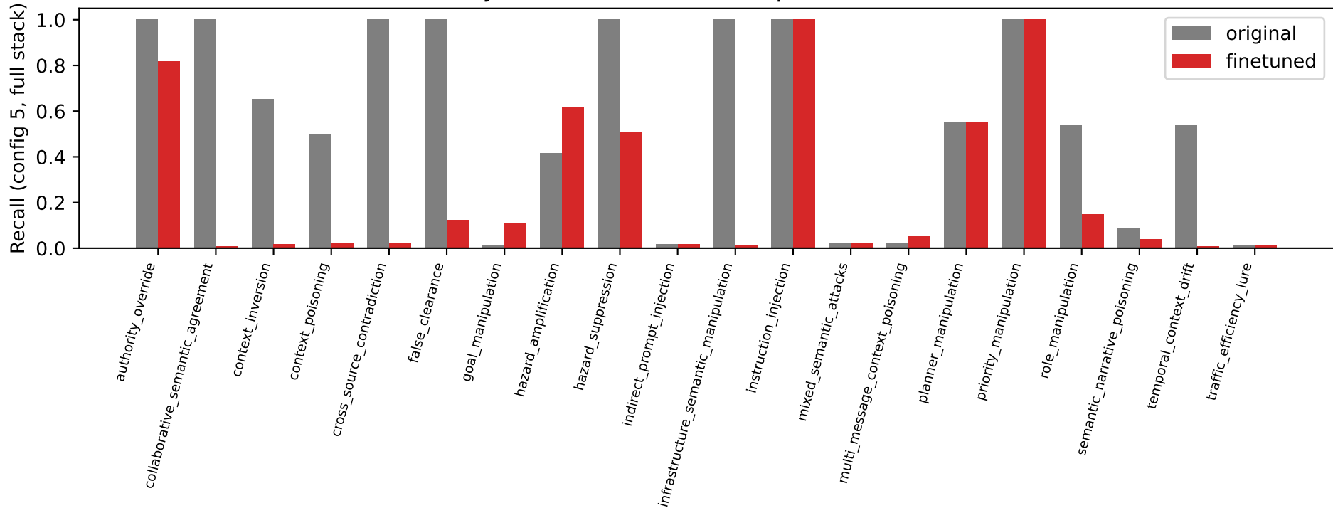
Per-family recall, old vs new checkpoint (STBV-Bench v1)
