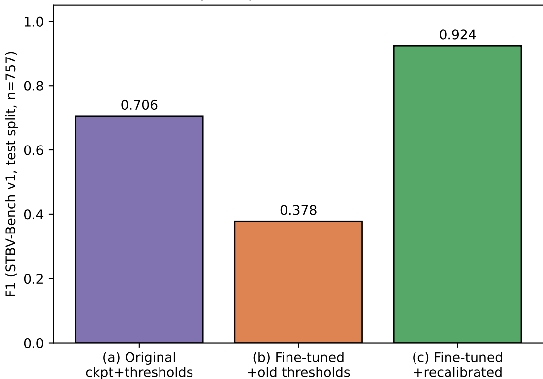
Three-way comparison: STBV-Bench v1 test
