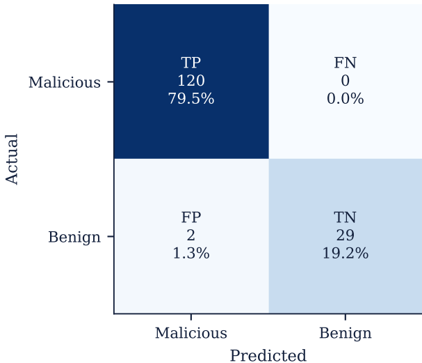
Confusion matrix ( \tau=0.5 )
