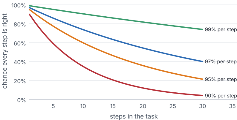
Figure 7.4. The chance that every step of a task goes right, for different per-step reliabilities. Small per-step error rates become large task failure rates as the number of steps grows.
