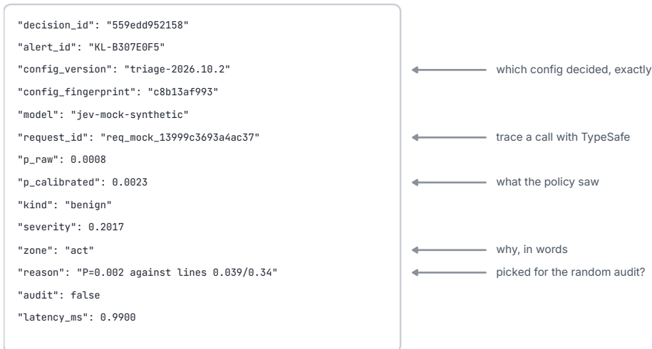
Figure 21.2. One decision record, with notes on why each field is there. Together they say what the service saw, what the model said, what the policy did, which version decided, and why.
