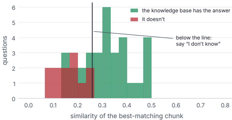
Figure 7.2. The similarity of the best-matching chunk, for questions the knowledge base can answer (green) and questions it can’t (red). They overlap, but not much. Below a threshold, the system should decline to answer.
