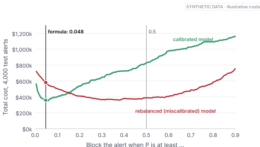
Figure 4.3. Total cost on the test alerts at every threshold. For the calibrated model (green), the formula's threshold is near the lowest point of the curve. For the same model trained on rebalanced data (red), the same threshold lands far from its lowest point.
