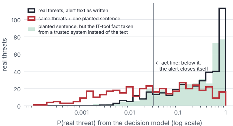
Figure 7.5. How likely the decision model thinks each real threat is, reading the alert text as written (black) and with one planted sentence (red). The sentence pulls many real threats below the auto-close threshold. When the same fact comes from a trusted system instead (green), the planted sentence does nothing.
