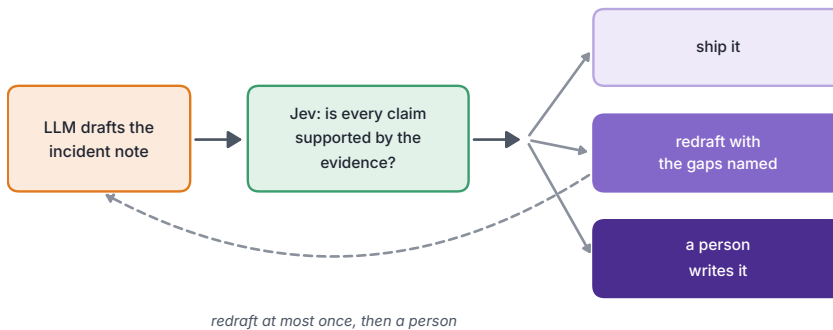
Figure 15.6. Check the writer. The LLM drafts; a decision model answers typed questions about the draft and the evidence together; the answer decides whether the draft is sent, goes back once to be rewritten, or goes to a person.
