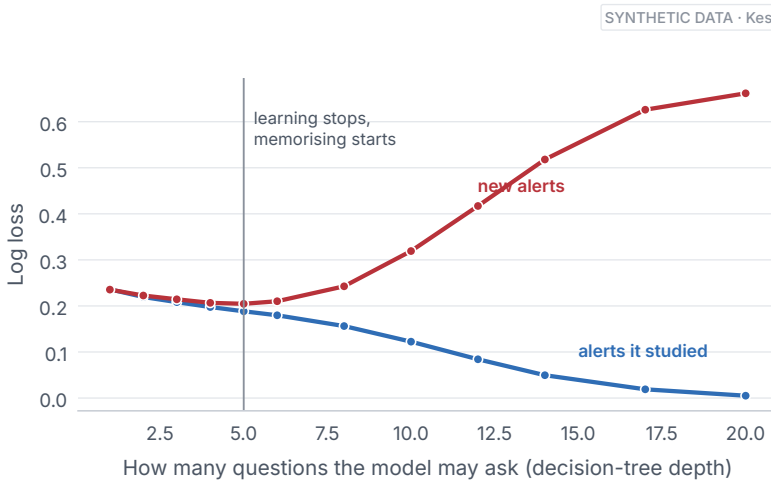
Figure 2.7. A decision tree allowed only a few questions learns general patterns. Allowed dozens, it memorises individual training alerts: its loss on them approaches zero while its loss on new alerts climbs.
