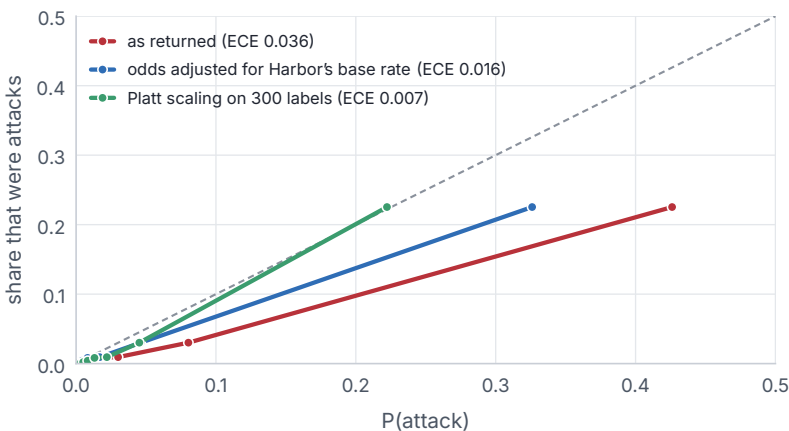
Figure 11.3. Harbor's alerts, on the cases not used for fitting: as returned (red), after adjusting the odds for Harbor's base rate (blue), and after Platt scaling on 300 labelled alerts (green). Both fixes bring the curve most of the way back to the diagonal.
