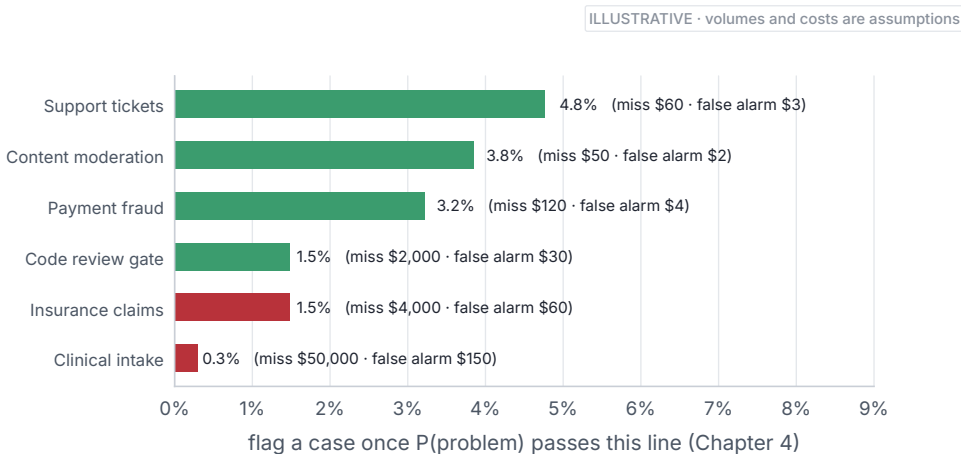
Figure 19.3. Where the threshold falls in each domain, from its (illustrative) costs of a miss and a false alarm. Support tickets flag at about 5%; clinical intake at about 0.3%. Same formula, different jobs.
