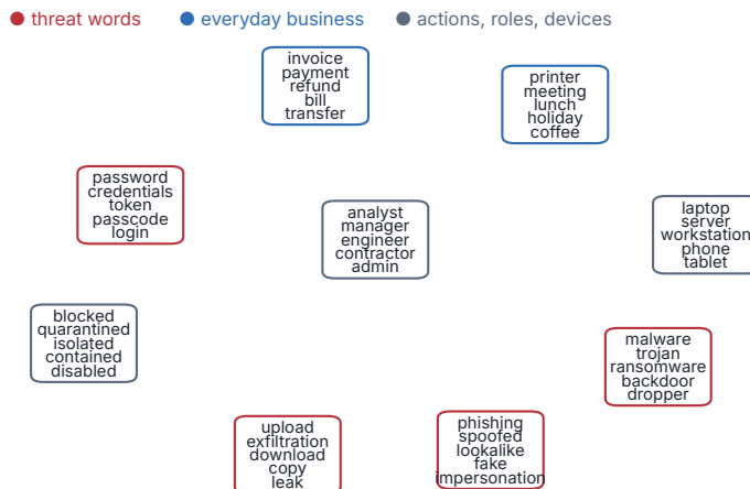
Figure 5.2. Word vectors learned from 30,000 synthetic analyst notes, with similar vectors placed close together. Each card is a family of words the method discovered on its own, from context alone: kinds of lure, kinds of malware, kinds of secret.
