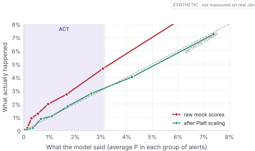
Figure 14.3. A close-up of the low end, where the act zone is. Raw scores (red) sit above the diagonal: the model was more confident than it should have been. After Platt scaling fitted on other days (green), the curve stays much closer to the diagonal.
