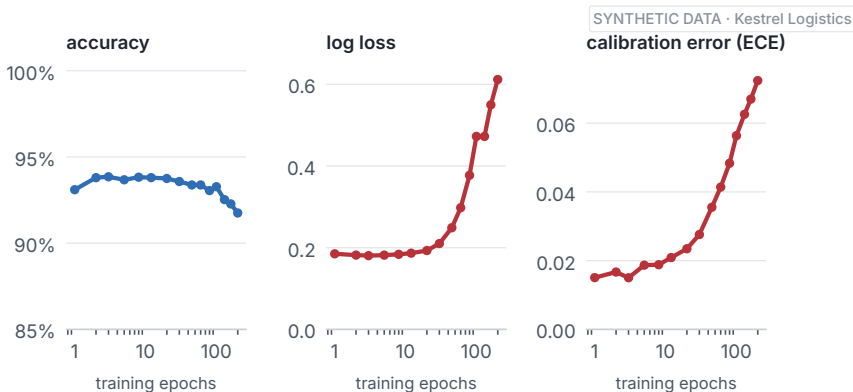
Figure 5.5. The same training run, on test alerts. Accuracy (left) barely moves. Log loss (middle) and calibration error (right) are flat for a while, then climb steeply. Watch only accuracy and you’d never notice.
