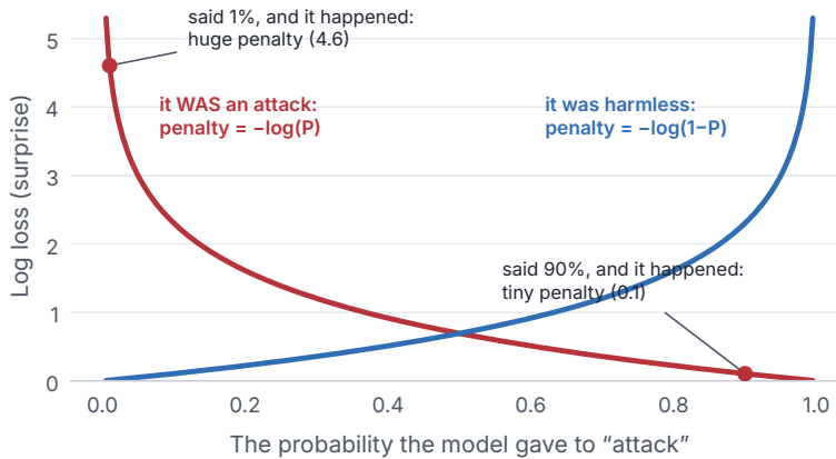
Figure 2.5. Log loss for a single alert. If it really was an attack (red), the penalty is small when the model gave “attack” a high probability. It grows very fast as that probability gets close to zero. Harmless alerts (blue) work the same way from the other side.
