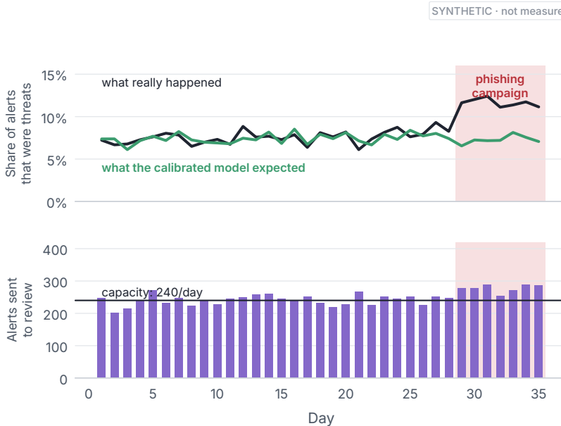
Figure 14.7. Top: the share of alerts that were real threats each day (black) against what the calibrated model expected (green). Bottom: alerts sent to review each day against the team's capacity. In week five (shaded), reality moves away from the model, and the queue overflows.
