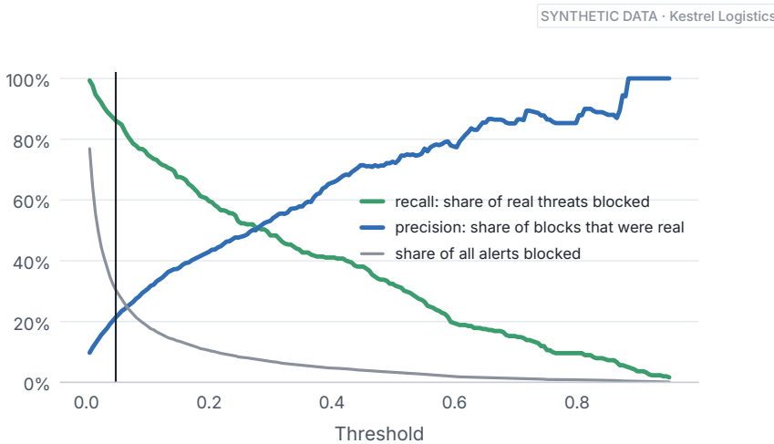
Figure 4.4. As the threshold moves up, precision (how many blocks were real) rises and recall (how many threats got blocked) falls. The grey curve shows how much traffic you're blocking. The vertical line is the cost-based threshold.
