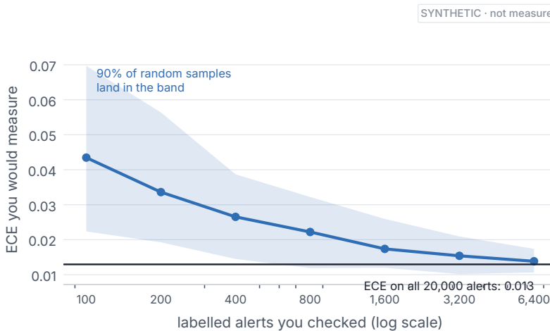
Figure 11.4. The ECE you'd measure from a random sample of labelled alerts, for different sample sizes, on a model whose ECE over all 20,000 alerts is shown by the black line. With a hundred labels the measurement is both noisy and too high on average: a calibrated model looks miscalibrated. The error shrinks as samples grow.
