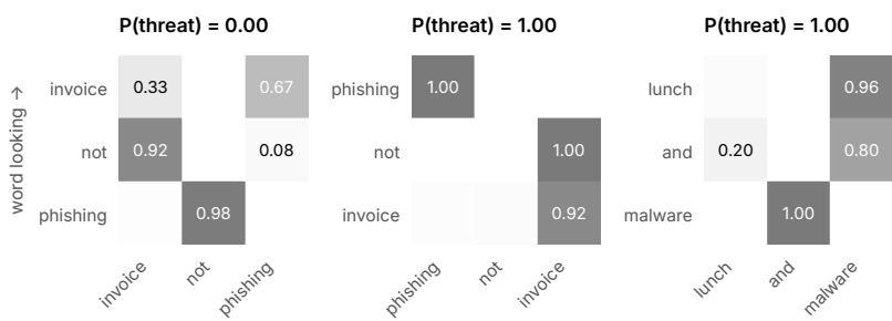
Figure 5.4. What each word attends to after training. In “invoice not phishing”, the word “phishing” puts nearly all its attention on “not”. Nobody told the model about negation; it found that looking at the word before was the cheapest way to get the answers right.
