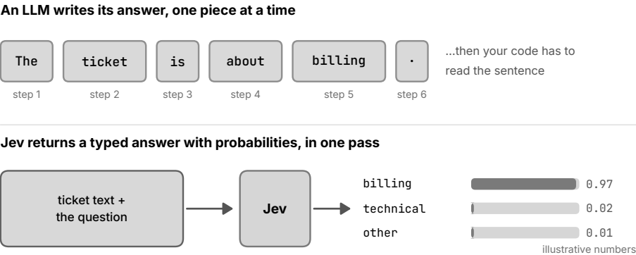
Figure 1.4. The same question, two ways. An LLM writes its answer out, piece by piece, and your code has to read the sentence. A decision model returns the answer as data, with a probability for every option, in one pass.
