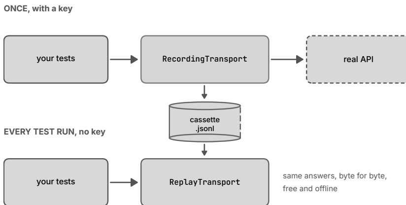
Figure 16.6. Record once, replay many times. With a key, a recording transport saves each real request and response to a file. In every later test run, a replay transport answers from that file: the same answers, byte for byte, with no key and no cost.
