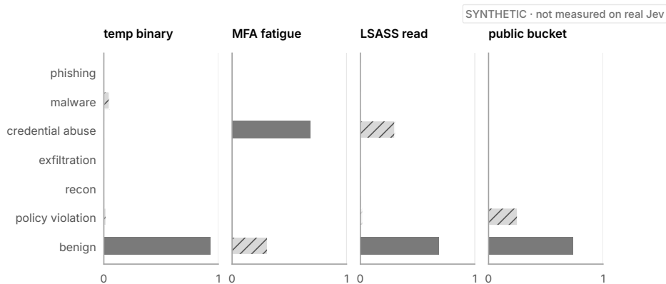
Figure 10.3. Category probabilities for four alerts. Some are clearly decided; others spread their probability over two or three labels. The spread is useful: it tells you how sure the model is, and which labels it’s choosing between.
