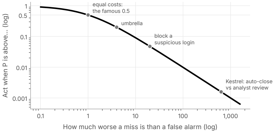
Figure 4.2. The right threshold for any ratio between the cost of a miss and the cost of a false alarm (both axes on a log scale). Equal costs give 0.5. As misses get more expensive, the threshold drops fast.
