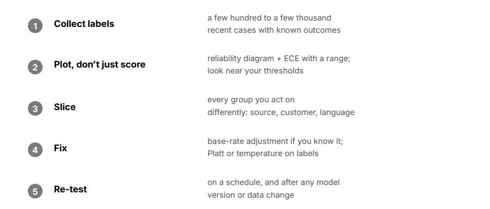
Figure 11.6. A testing routine for any model that returns probabilities, Jev included.
