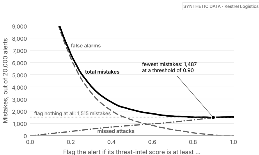
Figure 1.2. Every possible threshold, and the mistakes it makes. Low thresholds give the team far too many false alarms; high ones miss attacks. The total is lowest at the far right, just below the thin dotted line for “flag nothing at all”.
