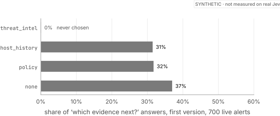
Figure 17.2. How often the first version of the agent chose each option at its “which evidence next?” step, across 700 live alerts. It never once chose threat intel.
