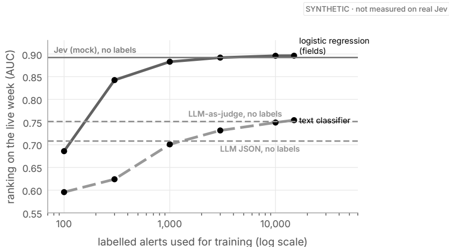
Figure 13.4. Ranking on the live week as the trained methods see more labelled alerts, averaged over random samples. Jev and the LLMs need no labels to start, so they’re flat lines. Logistic regression catches up with Jev at about 3,000 labels.
