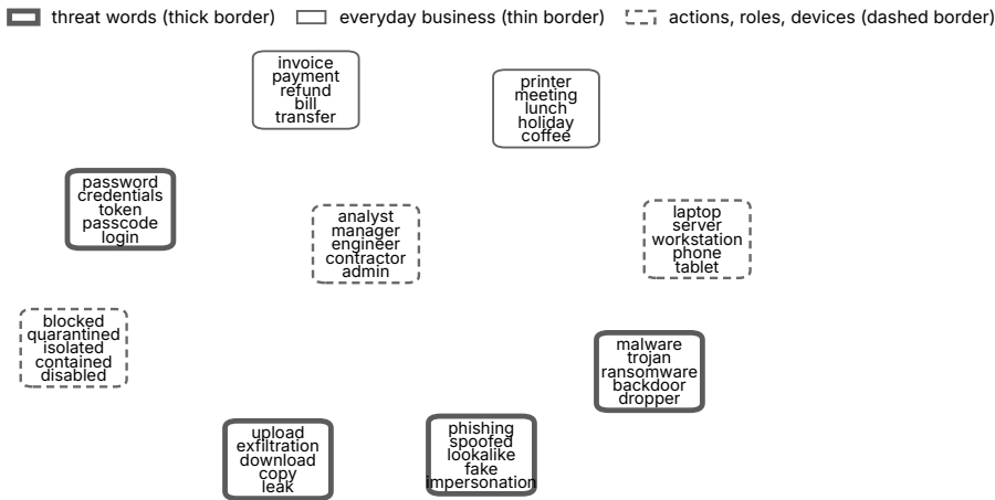
Figure 5.2. Word vectors learned from 30,000 synthetic analyst notes, with similar vectors placed close together. Each card is a family of words the method discovered on its own, from context alone: kinds of lure, kinds of malware, kinds of secret.
