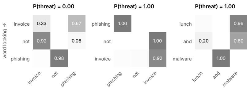
Figure 5.4. What each word attends to after training. In “invoice not phishing”, the word “phishing” puts nearly all its attention on “not”. Nobody told the model about negation; it found that looking at the word before was the cheapest way to get the answers right.
