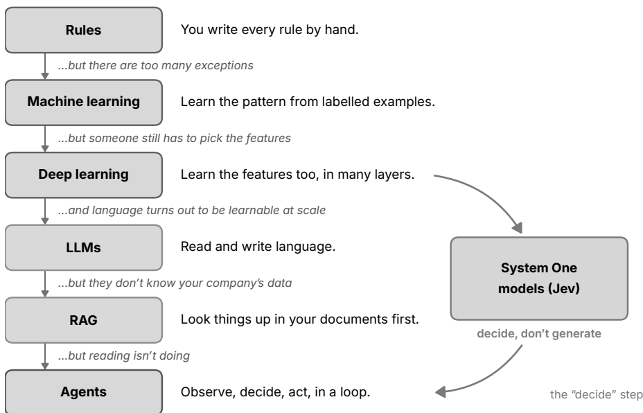
Figure 1.5. The story so far. Each step exists because the one before it hit a problem it couldn't solve. System One models like Jev grow out of deep learning and fit into the "decide" step of an agent.
