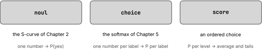
Figure 10.2. You’ve met each type before. A noul is the S-curve from Chapter 2, turning evidence into one probability. A choice is the softmax from Chapter 5, turning a score per label into a probability per label. A score is a choice whose labels come in order.
