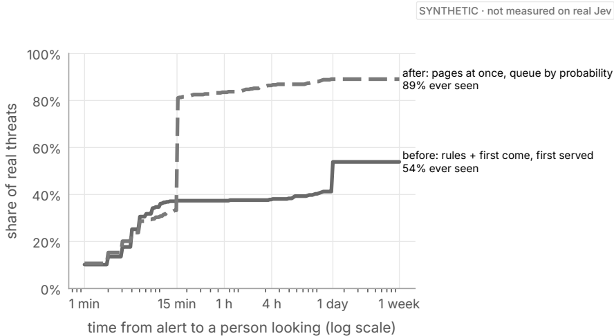
Figure 18.4. How long it takes for a real threat to reach a person. Before, rule-flagged threats were seen quickly and the rest waited up to a day or were never seen. After, urgent calls reach someone in about fifteen minutes and the queue takes the likeliest threats first.
