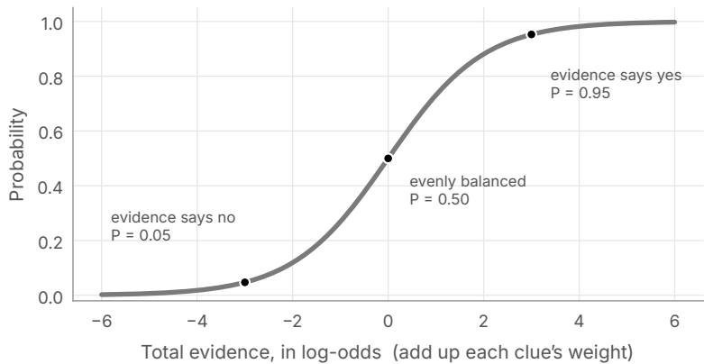
Figure 2.4. The S-curve (the logistic, or sigmoid, function) turns total evidence into a probability. Every step to the right multiplies the odds by the same amount, which is why the curve flattens out: once you’re very sure, more evidence changes the probability only a little.
