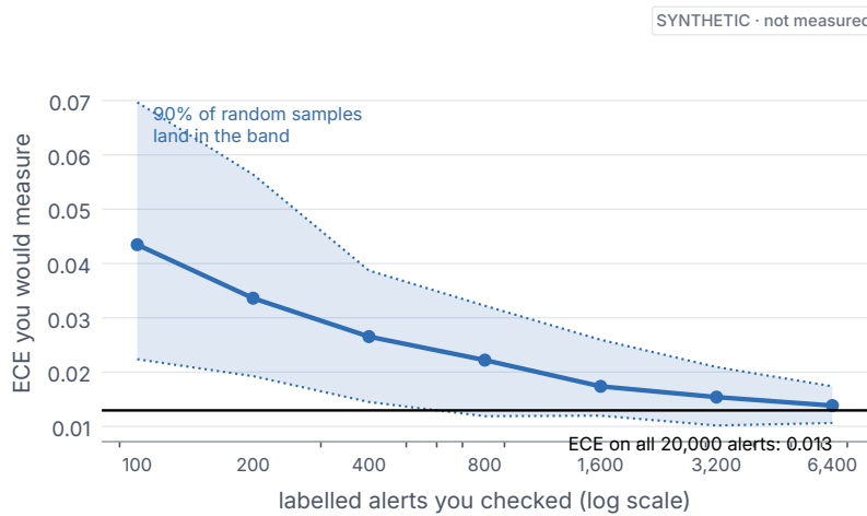
Figure 11.4. The ECE you’d measure from a random sample of labelled alerts, for different sample sizes, on a model whose ECE over all 20,000 alerts is shown by the labelled black horizontal line. With a hundred labels the measurement is both noisy and too high on average: a calibrated model looks miscalibrated. The error shrinks as samples grow.
