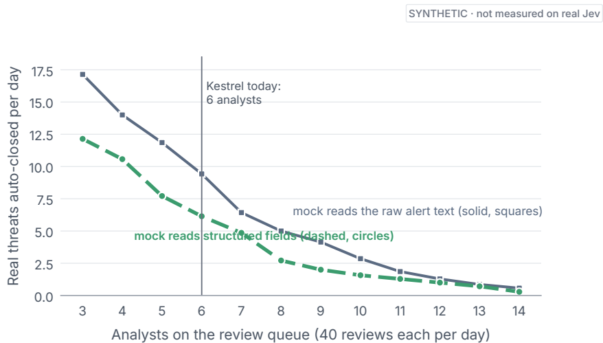
Figure 14.5. Threats auto-closed per day, for every team size from 3 to 14 analysts, with thresholds fitted again for each. The gap between the two curves is what better input is worth: the same model reading structured alert fields instead of raw alert text.
