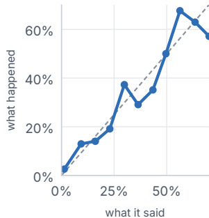
TinyJev as trained ECE 0.017
