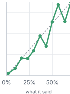
after temperature ECE 0.009
