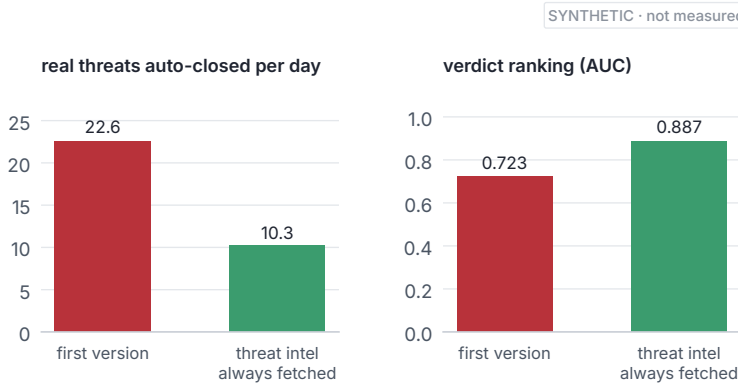
Figure 17.3. The same agent before and after one change: always fetching threat intel. Real threats auto-closed per day fell by more than half, and the verdict's ranking recovered.
