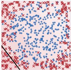
one neuron
