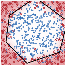
3 hidden neurons
