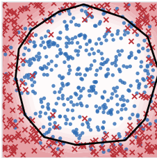
12 hidden neurons
