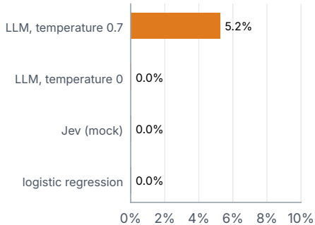
verdict changes across 5 identical calls
