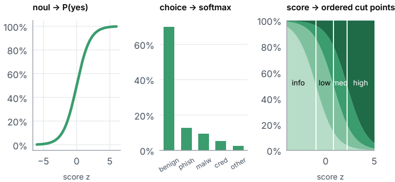
Figure 20.2. The three heads. A noul turns one number into P(\text{yes}) with the S-curve. A choice turns one number per label into probabilities that add up to 1. A score turns one number into probabilities for levels in order, by cutting it at points that must stay in order.
