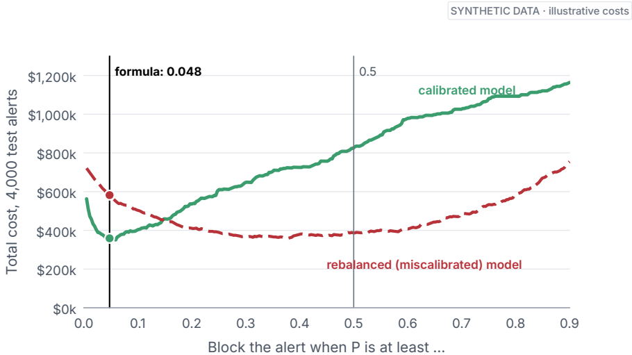
Figure 4.3. Total cost on the test alerts at every threshold. For the calibrated model (green, solid line), the formula's threshold is near the lowest point of the curve. For the same model trained on rebalanced data (red, dashed line), the same threshold lands far from its lowest point.
