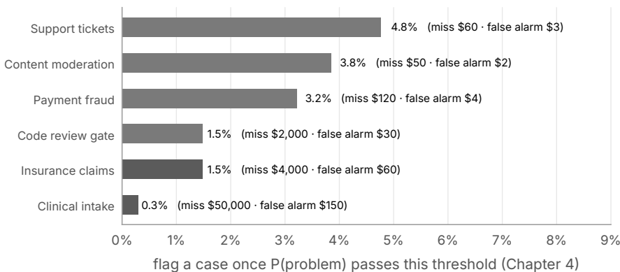
Figure 19.3. Where the threshold falls in each domain, from its (illustrative) costs of a miss and a false alarm. Support tickets flag at about 5%; clinical intake at about 0.3%. Same formula, different jobs.
