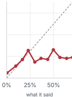
the overtrained net ECE 0.069
