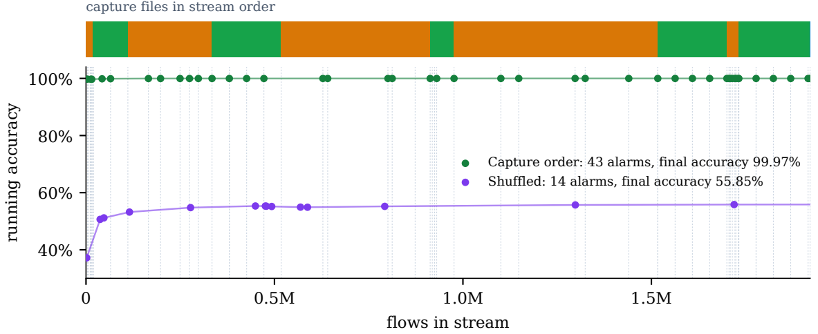
Figure 3: ADWIN drift alarms over the 1,921,182-flow stream. Top band: the 58 capture files present in this stream, in order, coloured by attack family (green volumetric, orange reconnaissance, grey low-rate, blue benign); dashed lines are file seams. In capture order the alarms sit on the seams and running accuracy stays near 100%; the same model on the shuffled stream alarms 14 times and finishes at 55.9%.
