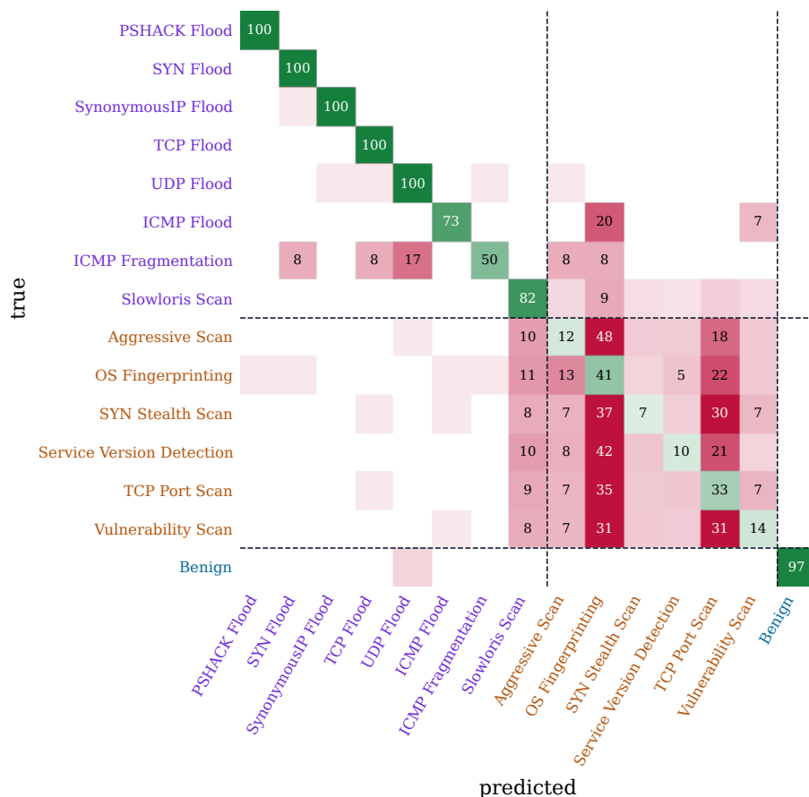
Figure 4: Random Forest confusion matrix, each row normalised and averaged over the three seeds (percentages; cells under 5% unlabelled). Dashed lines separate denial of service, reconnaissance and benign. The other three models are on the dashboard’s Findings tab.
