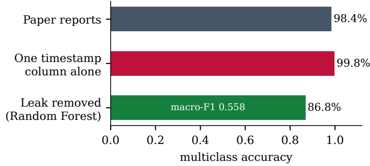
Figure 2: The contribution in one chart, all as multiclass accuracy. A single capture-timestamp column beats the published model; with the leak removed the Random Forest scores 86.8% accuracy and macro- F_1 0.558, the honest figure because it weights every class equally.
