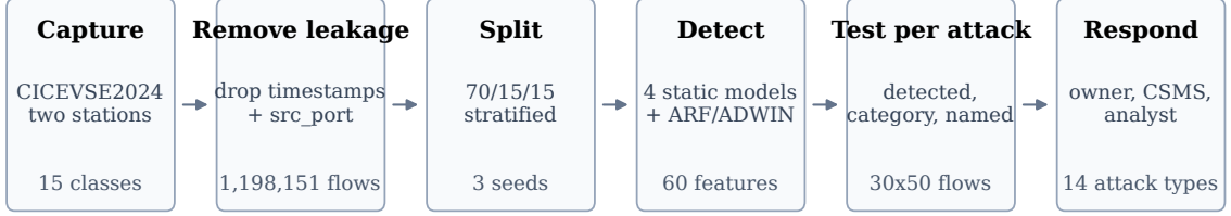
Figure 1: Method at a glance. Numbers are read from the exported results; the same diagram heads the project’s /docs page.
