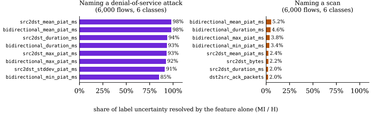
Figure 5: For each feature, the share of the uncertainty about which attack a flow is that the feature removes on its own ( I(X_j; Y)/H(Y) ), computed separately inside denial-of-service and inside reconnaissance flows (6,000 held-out flows each, seed 42, k -NN mutual-information estimator). Both panels share one axis.
