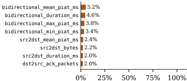
Naming a scan (6,000 flows, 6 classes)
