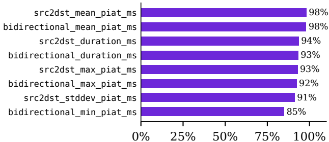
Naming a denial-of-service attack (6,000 flows, 6 classes)
