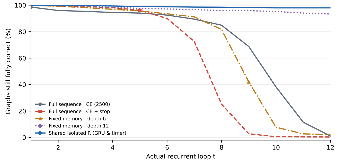
One fixed prompt: Steps = 256
