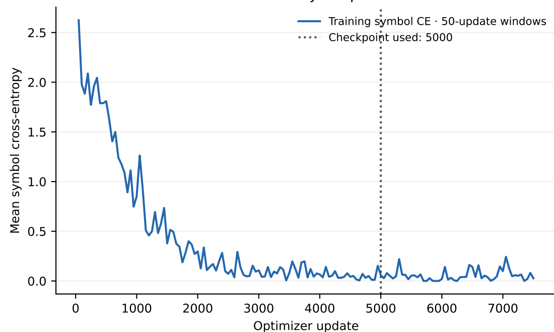
Fixed memory · depth 12
