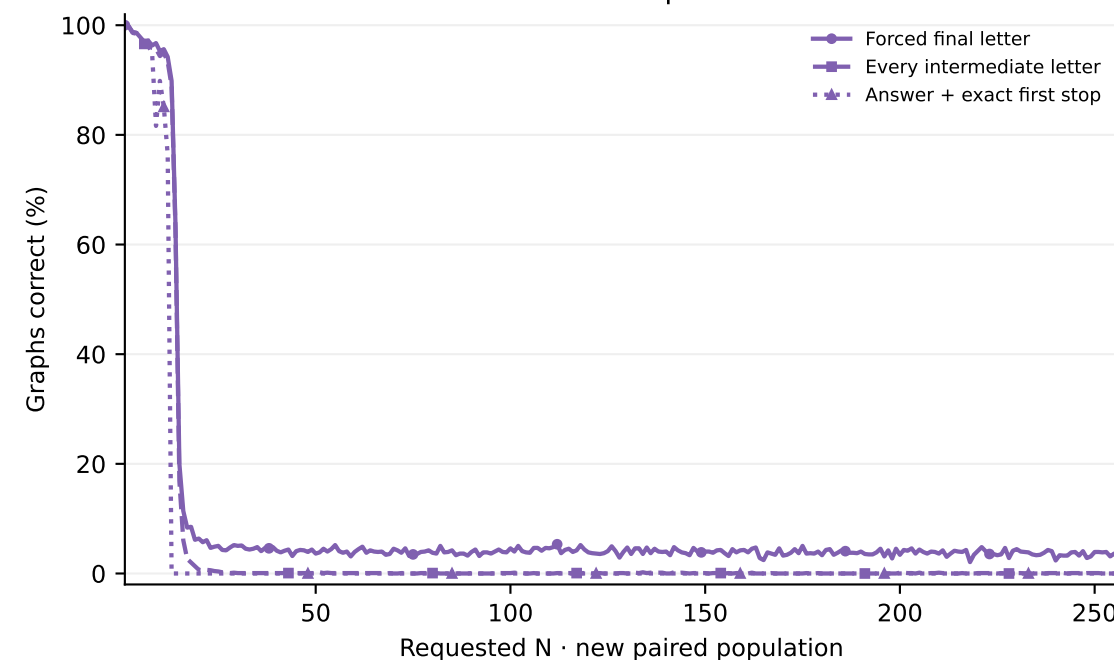
Frozen selected-checkpoint evaluation
