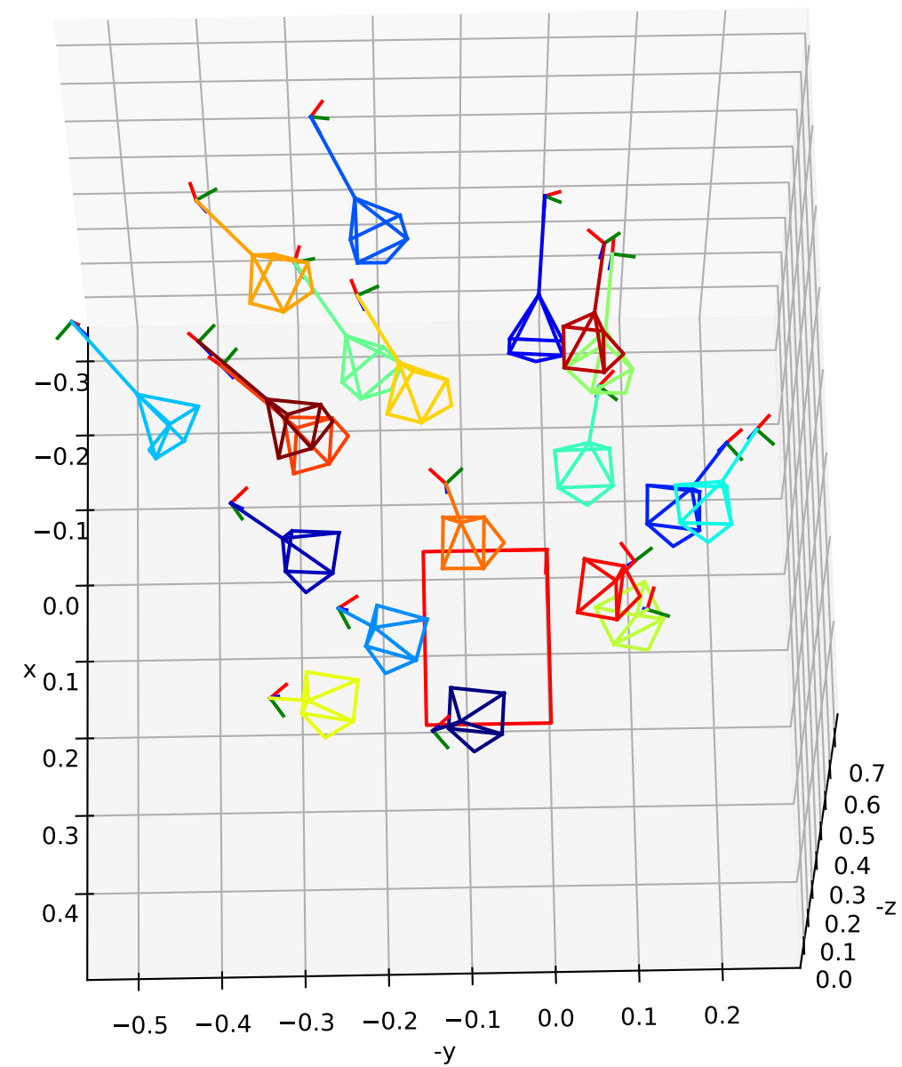
Hand-Eye Calibration Visualization
