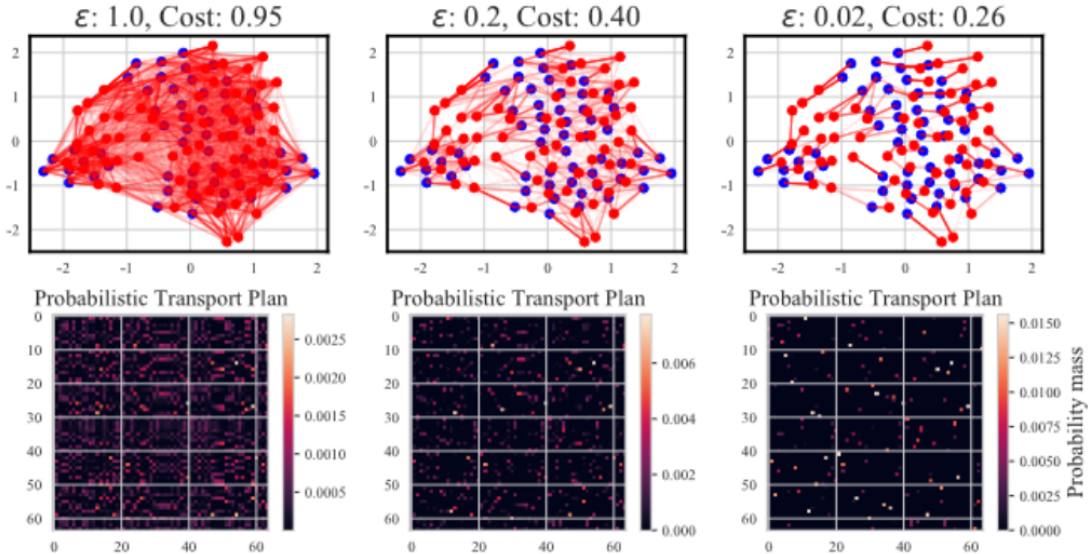
Figure 3: Regularization controls how much 'spread out' the mass is, since we bias the optimization towards the product measure which is 'the most spread out'.
