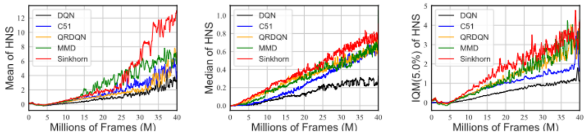
Figure 4: Atari performance for all methods covered. The three panels show the mean, median, and interquartile mean of human-normalized scores over training. Results taken from [BDR23]
