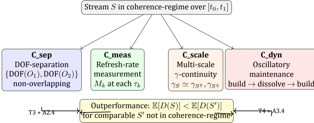
Figure .7: The four conditions of the Coherence Principle (Definition 5.1.1, Propositions 5.2.1–5.2.4). Each condition is derived from an axiom/theorem clause (italic text below each box). The joint sufficiency (Prop 5.2.5) is the downstream arrows to the outperformance inequality (Theorem 5.1.2).
