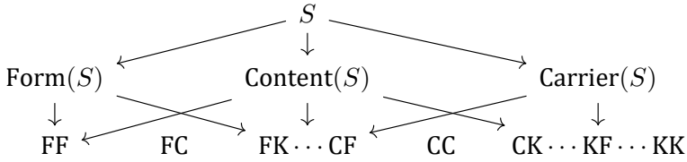
Figure .3: Recursive Triple-decomposition at depth 2. Each of \text{Form}(S) , \text{Content}(S) , \text{Carrier}(S) is itself a stream, so the Triple functor applies again, yielding nine depth-2 components (abbreviated: \text{FF} = \text{Form}(\text{Form}(S)) , \text{FC} = \text{Content}(\text{Form}(S)) , etc.). Finite-depth iteration is well-defined for every adequate F -coalgebra (Lemma 6.3.2). Full \omega -depth requires additional hypotheses (H1, H2; §6.9).
