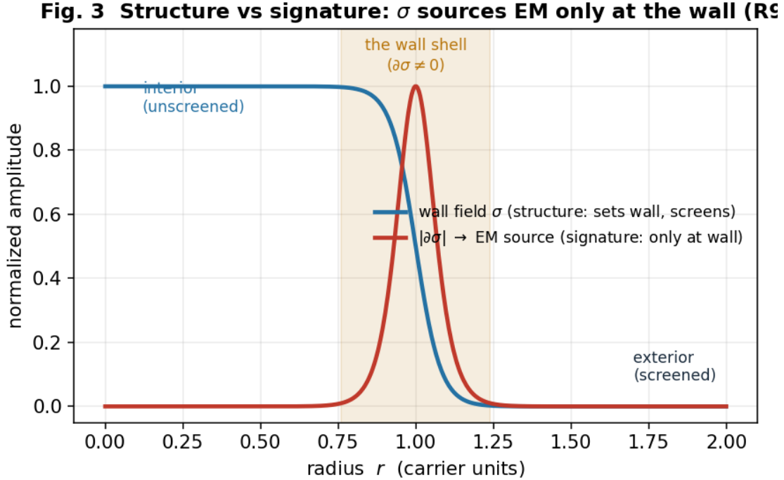
Fig. 3 — Structure versus signature (R9). The screened wall field \sigma (structure: sets the wall, screens, derives place-fixedness) and its electromagnetic signature |\partial\sigma| , which is nonzero only on the wall shell — the EM source is sourced by the wall field at the wall, by the field equations.
