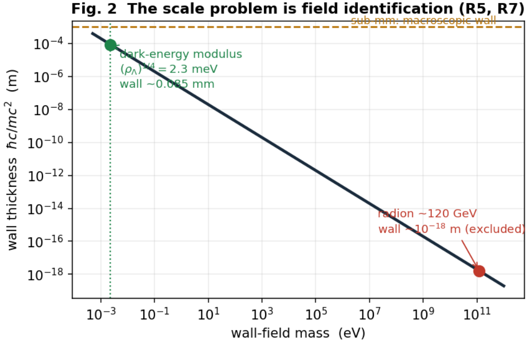
Fig. 2 — The scale problem is field identification (R5, R7). Wall thickness hc/mc^2 versus field mass: the radion (sub-nuclear wall, excluded for a macroscopic portal) versus the meV dark-energy modulus (0.085 mm wall, macroscopic), with the (\rho_\Lambda)^{1/4} = 2.3 meV line and the sub-mm macroscopic threshold.
