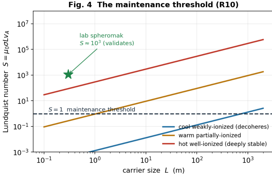
Fig. 4 — The maintenance threshold (R10). Lundquist number S = \mu_0 \sigma L v_A versus carrier size for cool, warm, and hot/ionized regimes, with the S = 1 self-maintenance threshold and the laboratory-spheromak validation point ( S \approx 10^3 ).
