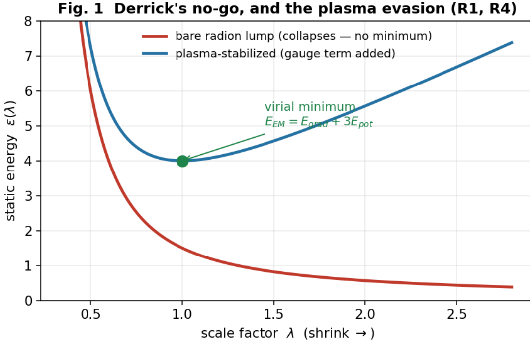
Fig. 1 — Derrick's no-go, and the plasma evasion (R1, R4). \varepsilon(\lambda) for the bare radion lump (monotone collapse, no stationary point) versus the plasma-stabilized configuration (a genuine minimum at the virial point E_{EM} = E_{grad} + 3E_{pot} ).
