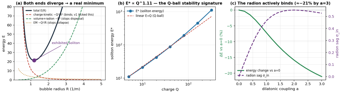
Fig. 6 — The gauged dilatonic Q-ball, exhibited (R12). (a) The energy E(R) diverges at both ends — the charge-kinetic binding term ( Q^2/R^3 ) stops dispersal, the electromagnetic term ( Q^2/R ) stops collapse — leaving a genuine soliton minimum. (b) The soliton energy grows linearly with charge, E \propto Q^{1.1} , the Q-ball stability signature. (c) The radion sags ( \sigma_{in} ) and lowers the soliton energy by up to 21 % as the dilatonic coupling a increases — the dark-energy-scale field actively binds the configuration.
