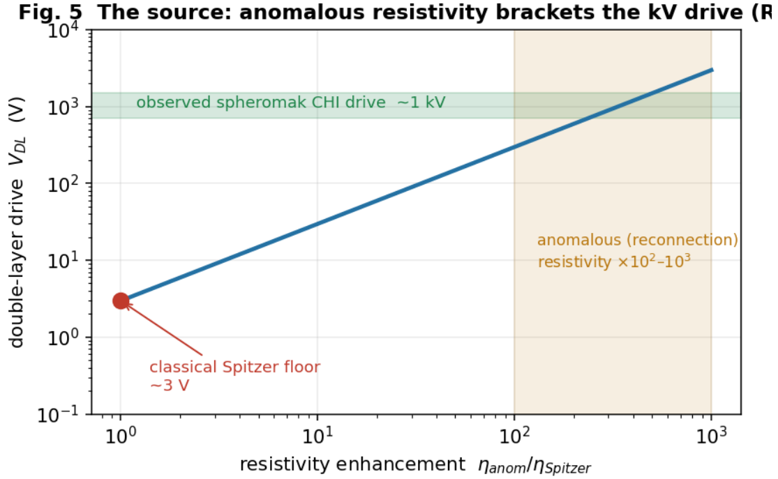
Fig. 5 — The source: anomalous resistivity brackets the kV drive (R11). Double-layer drive potential versus resistivity enhancement: the few-volt classical Spitzer floor rises through the \times 10^2-10^3 anomalous-(reconnection)-resistivity band to bracket the observed 1 kV spheromak coaxial-helicity-injection drive.
