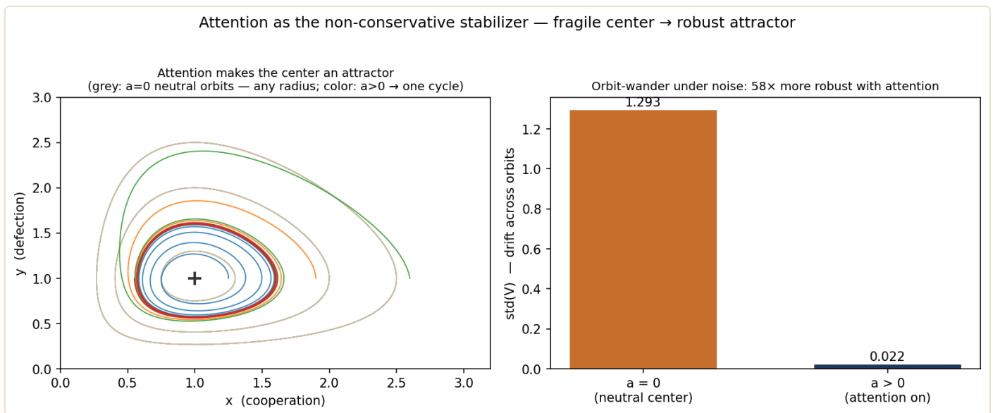
Figure 7. Attention is the non-conservative stabilizer. Left: with attention off ( a = 0 ) the bare center is neutral — a continuum of orbits (grey), any of which noise can drift between; with attention on ( a > 0 ) trajectories from every starting radius collapse onto one attracting cycle (color). Right: under identical stochastic perturbation, the drift across orbits shrinks by roughly fiftyfold once attention is on. The loop is robust precisely because the driving force does work — it is not conservative.
