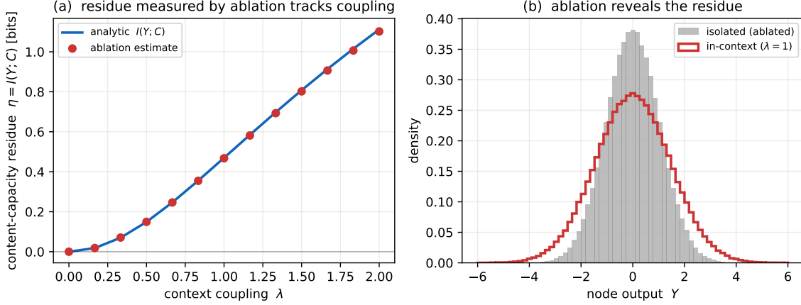
Figure 4: The residue is measurable by ablation in a running classical system. Illustrative simulation of a node S with output Y = X_{\text{own}} + \lambda C + \text{noise} , where C is the context delivered over the bus and \lambda the coupling. (a) The residue \eta = I(Y; C) , estimated by ablation (red points: empirical mutual information from comparing in-context and isolated output samples), tracks the analytic Gaussian value (blue line) and goes to zero as coupling \rightarrow 0 . (b) At \lambda = 1 , the node’s output distribution in-context (red) is broader than when isolated (grey); the divergence between them is exactly what the ablation measures — the context written into the part. This is the classical, deployment-ready companion to the quantum computation of Fig. 2.
