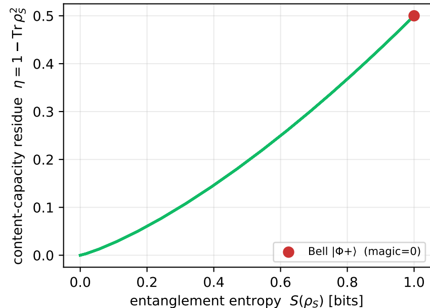
(a) residue tracks entanglement
