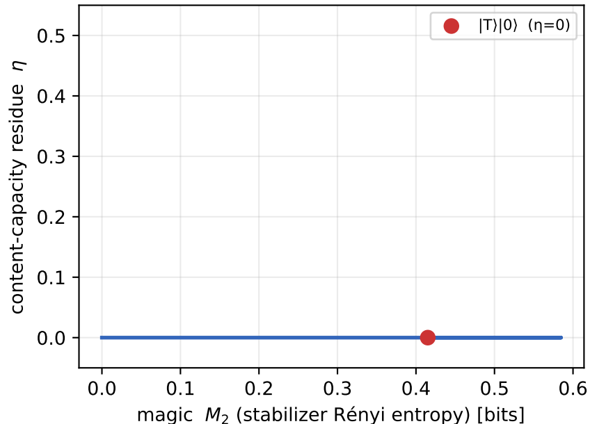
(b) residue is independent of magic
