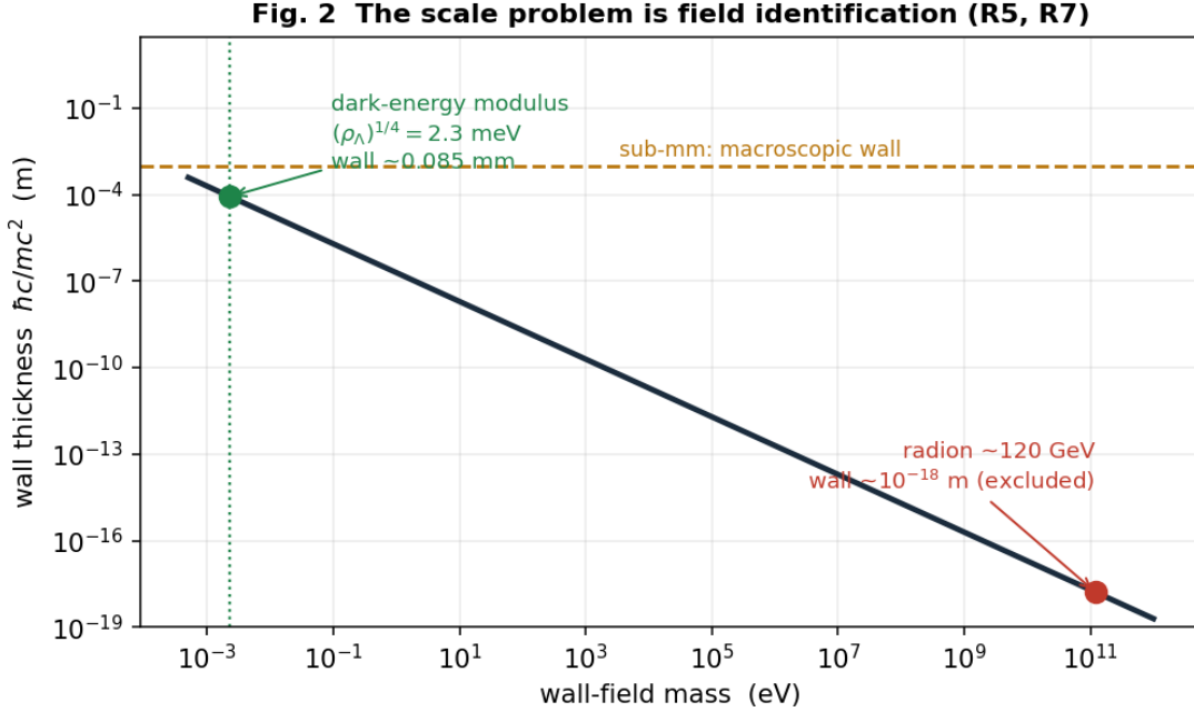
Fig. 2 — The scale problem is field identification (R5, R7). Wall thickness \hbar c/mc^2 versus field mass: the radion (sub-nuclear wall, excluded for a macroscopic portal) versus the meV dark-energy modulus (0.085 mm wall, macroscopic), with the (\rho_{\Lambda})^{1/4} = 2.3 meV line and the sub-mm macroscopic threshold.
