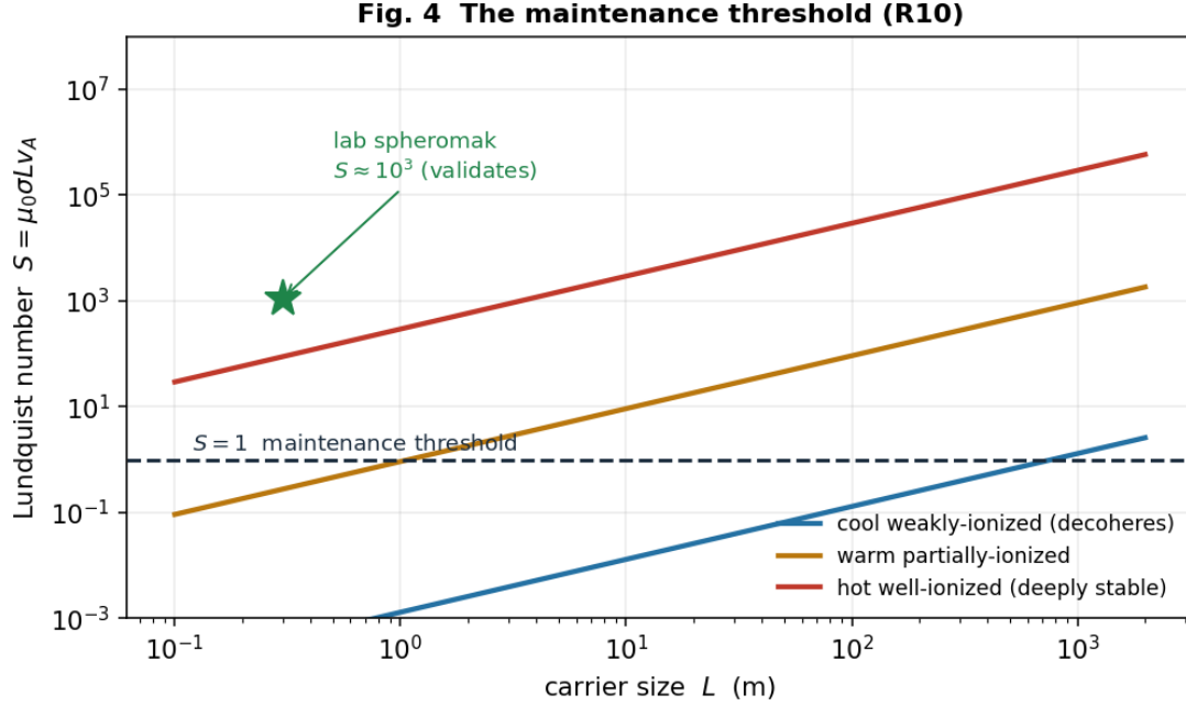
Fig. 4 — The maintenance threshold (R10). Lundquist number S = \mu_0 \sigma L v_A versus carrier size for cool, warm, and hot/ionized regimes, with the S = 1 self-maintenance threshold and the laboratory-spheromak validation point ( S \approx 10^3 ).
