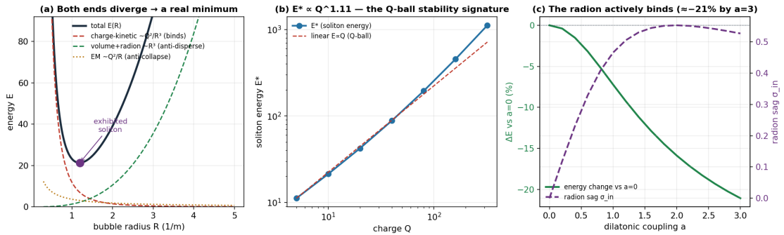
Fig. 6 — The gauged dilatonic Q-ball, exhibited (R12). (a) The energy E(R) diverges at both ends — the charge-kinetic binding term ( Q^2/R^3 ) stops dispersal, the electromagnetic term ( Q^2/R ) stops collapse — leaving a genuine soliton minimum. (b) The soliton energy grows linearly with charge, E \propto Q^{1.1} , the Q-ball stability signature. (c) The radion sags ( \sigma_{in} ) and lowers the soliton energy by up to 21 % as the dilatonic coupling a increases — the dark-energy-scale field actively binds the configuration.
