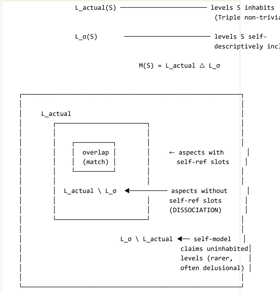
Figure 1.3 — The mismatch condition
