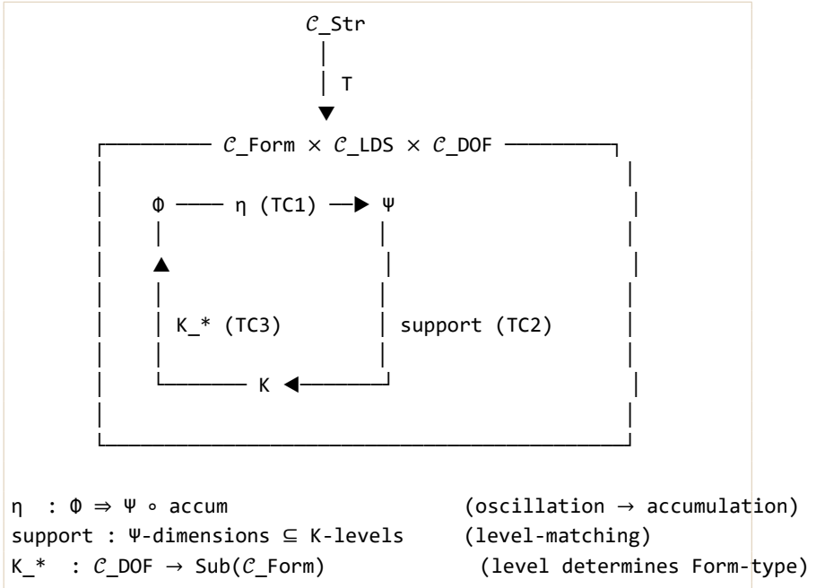
Figure 1.1 — The Triple as colax-limit diagram
