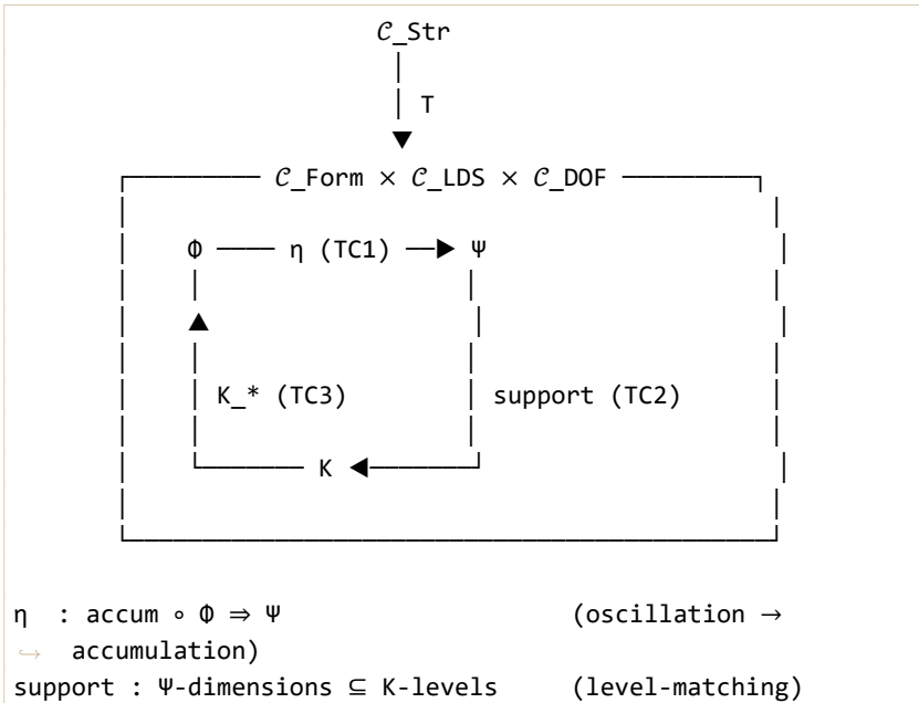
Figure 1.1 — The Triple as colax-limit diagram
