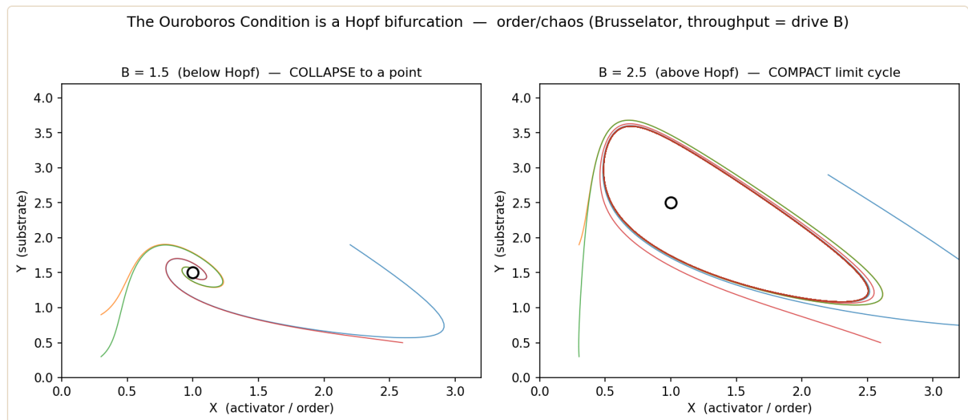
Figure 5. The Ouroboros Condition is a Hopf bifurcation. Order/chaos as the Brusselator: below a throughput threshold the polarity collapses to a point (left, the equilibrium sink — no sustained order); above it, the same dimension is a compact limit cycle (right, sustained order). The point blooms continuously into the circle as the throughput crosses the line — superposition and collapse as the two sides of one bifurcation.
